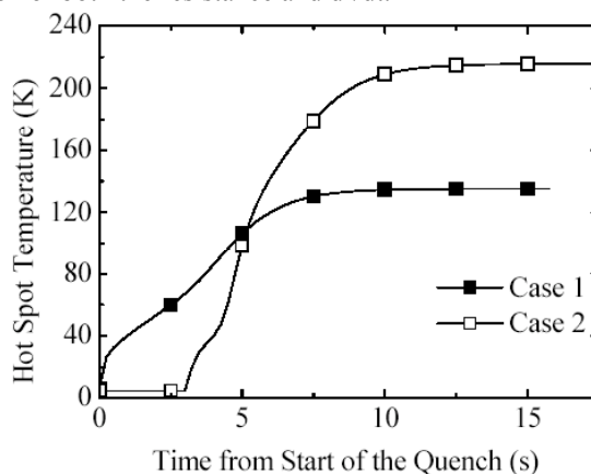
Fig. 5. Peak Hot Spot Temperature versus Time and Quench Velocities
